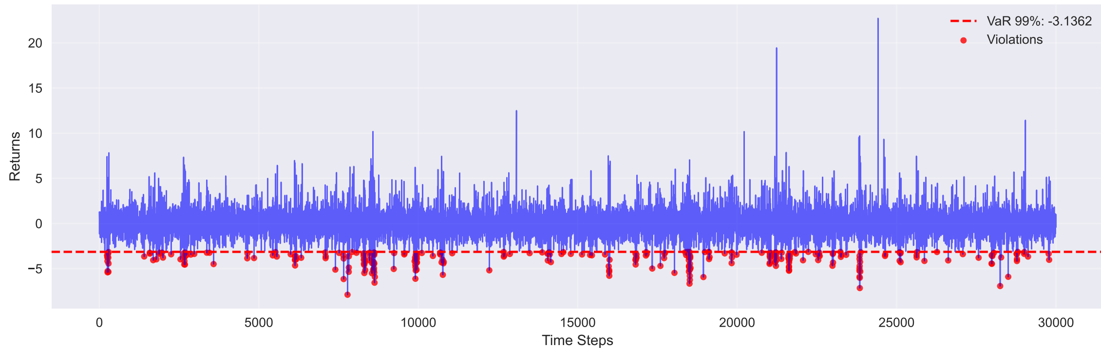
Zero Conditioned: VaR 99% Exceedance Timeline
